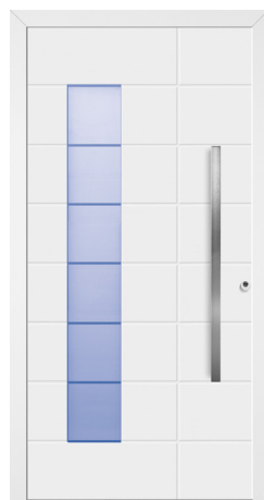
Motif 867 Ud = 0.9 (W/m 2 .K)
